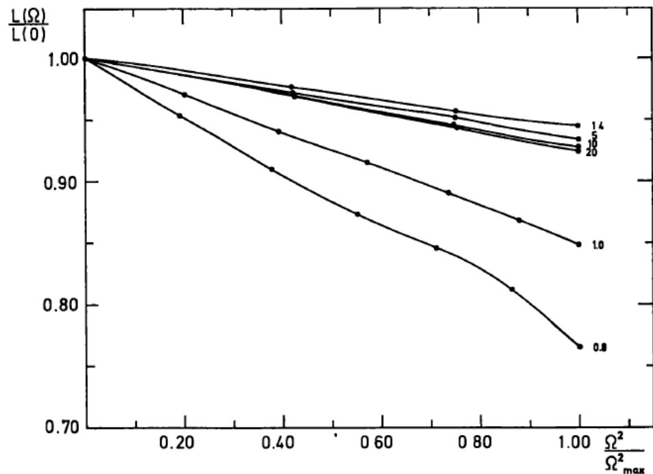
Fig. 1. The decrease of the luminosity with increasing rotation measured by \Omega^2/\Omega_{\max}^2 , where \Omega refers to the angular velocity of rotation and the subscript max to the critical case. The Arabic numeral refers to the mass of each sequence in solar units
