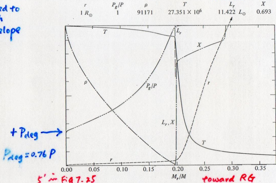
Fig. 7-26B A Model of Mass 1 M_\odot during the Subgiant Stage at t = 10.8747 \times 10^9 Years. Radius r , ratio P_g/P of gas pressure computed from the perfect gas law to the actual pressure with degeneracy included, temperature T , net luminosity L_r , and hydrogen abundance X are shown as functions of fractional mass M_r/M in the range 0 to 0.38. The distribution of L_r is a step function rising from zero to maximum scale with the initial rise in X . The lower limit of the ordinate is zero for all variables. The upper limits, given in the figure, are 1 R_\odot (with R_\odot = 6.96 \times 10^{10} cm; however, the total radius is 6.1784 R_\odot ), unity for the ratio of pressures, central density \rho_c ( \text{gm cm}^{-3} ), central temperature T_c ( ^\circ\text{K} ), total luminosity L (units of L_\odot = 3.86 \times 10^{33} erg \text{sec}^{-1} ), and hydrogen abundance X = 0.693 . The central pressure (not shown) is 6552.2 \text{ dyne cm}^{-2} . The time is measured from the initial model calculated for the pre-main-sequence phase (see Section 2). [Adapted from I. Iben, Jr., 1967 (326).]
