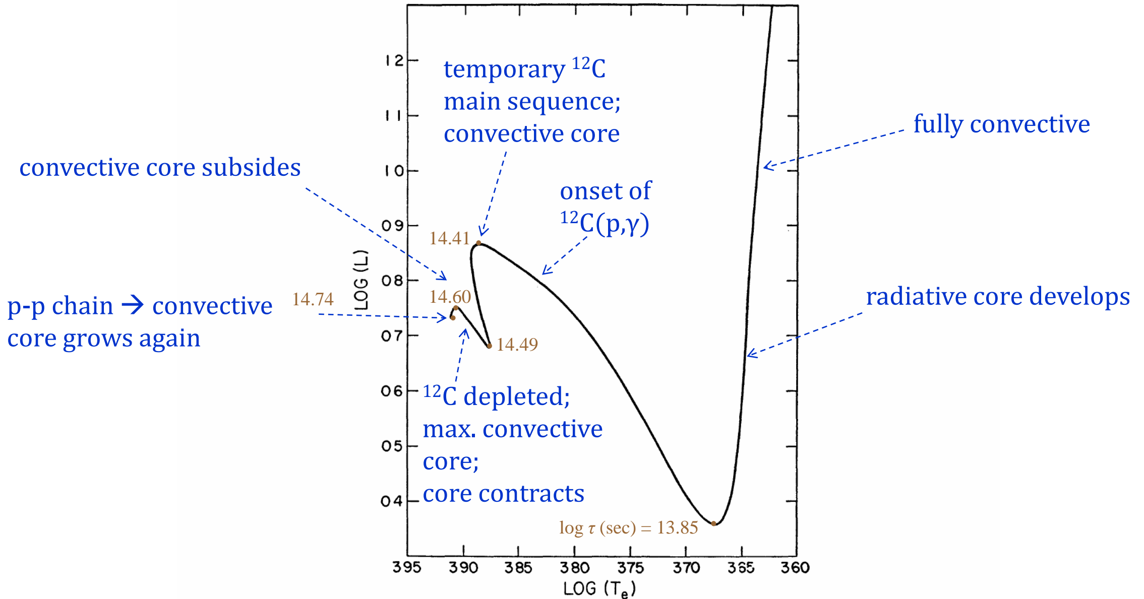
FIG. 6 —The path in the Hertzsprung-Russell diagram for M = 1.5 M_{\odot} . Units of luminosity and surface temperature are the same as in Fig. 1.
