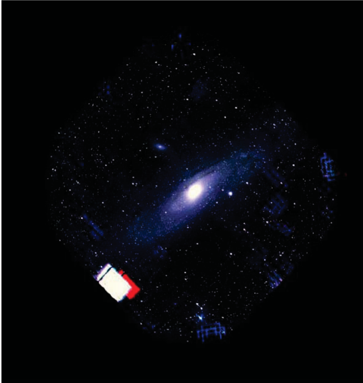
M31: full GPC1 FOV and a zoomed portion of the FOV
