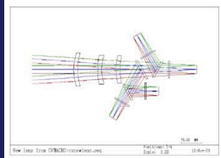
Optical Design
