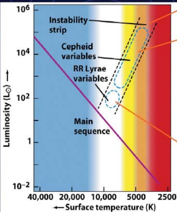
Figure 12-28 Discovering the Universe, Seventh Edition © 2006 W.H. Freeman and Company
