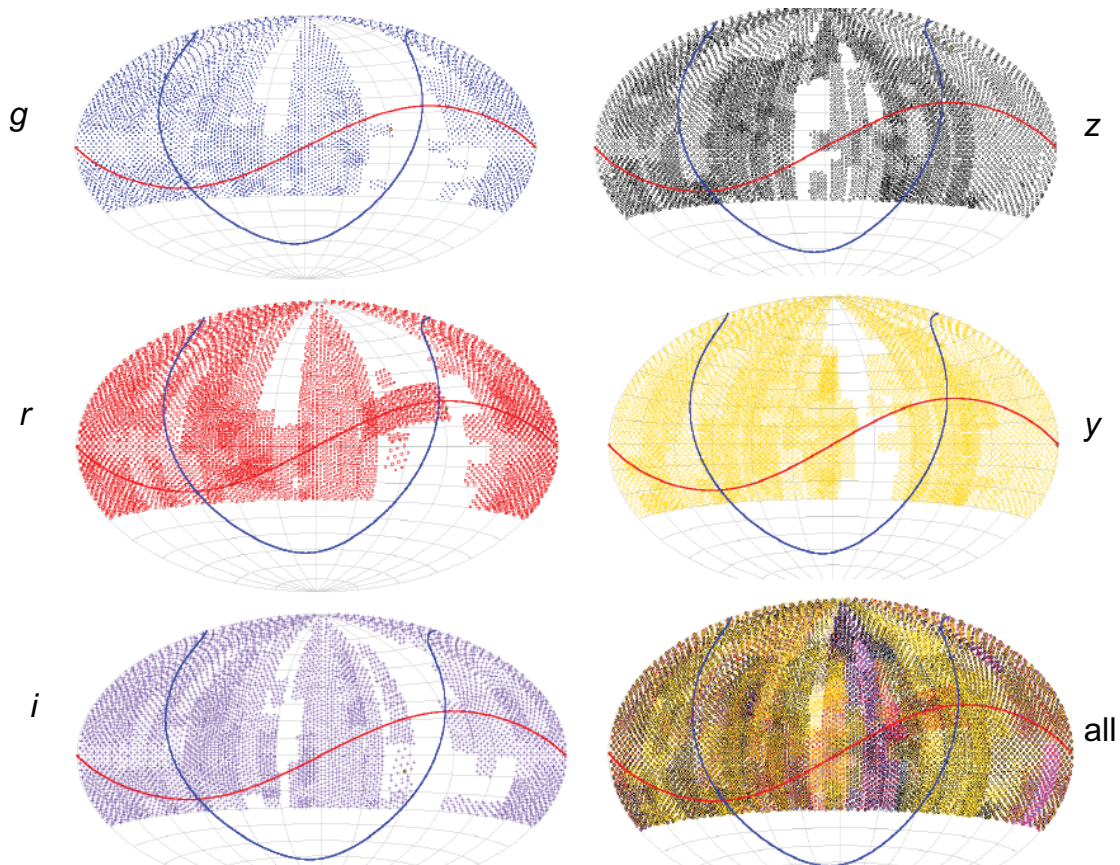
PS1 Sky Coverage as of 01Dec, 2010
