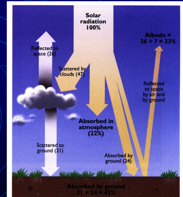
Figure 3. The interaction of sunlight with the atmospheric gases, clouds, and surface of Earth has many avenues. Ultimately, about one-third of the solar energy reaching our globe is reflected back to space.
