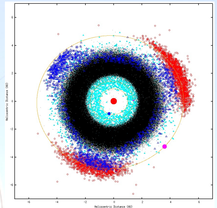
The inner Solar System
